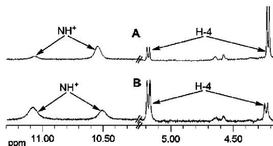
Figure 4. Partial ^1\text{H} NMR spectrum, including two sets of distinct protons at nitrogen and C-4, of TFA salt ( 1a ) of calyphaphinone in \text{CDCl}_3 . (A) Spectrum recorded at 298 K soon after TFA was added. (B) Spectrum recorded at 298 K after the solution was heated at 333 K for 20 min.
