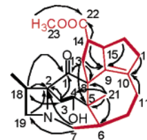
Figure 1. Key 1 H– 1 H COSY (—) and HMBC (---) correlations of calyphaphninone ( 1 ).
