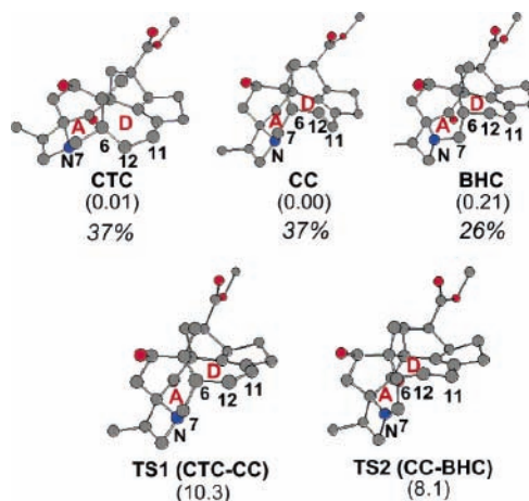
Figure 3. Three DFT-calculated minimum energy conformers (CTC, CC, and BHC) and two connecting TS (TS1 and TS2) found for calycephalinone ( 1 ). Free energies in kcal/mol relative to the stablest conformer CC are given in parentheses. Populations of three conformers (in italics ) are also given.
