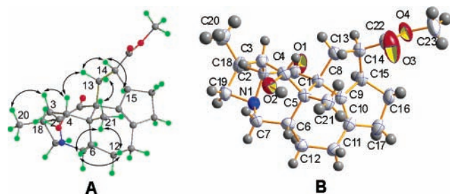
Figure 2. (A) Key ROESY correlations of 1 . (B) Single-crystal X-ray structure of 1 , in which C-11 and C-12 took upside and downside orientation, respectively, and the nitrogen lone pair pointed downside.
