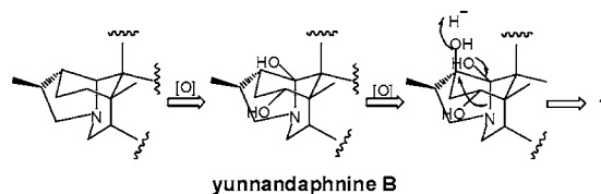
Scheme 1. Biogenetic Pathway Proposed for Calyphaphinone ( 1 )
